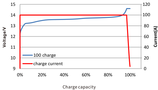
12V100Ah charge characteristics 0.5C @RT
