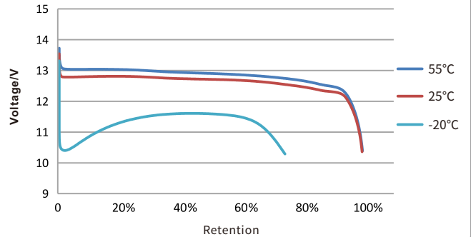
12V100Ah discharge curves at different temperatures
