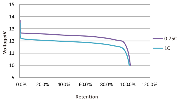
12V100Ah discharge curves at different rates@RT
