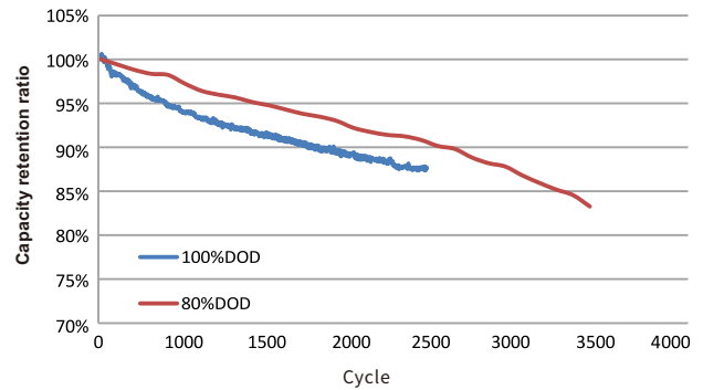
12V100Ah different DOD 0.5C cycle life curve @RT
